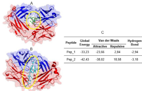
Figure 3. Visualization of 3D structure of the molecular docking analysis used PyMol software (https://pymol.org/2/). A. Pep_1 vs BCR; B. Pep_2 vs BCR; C. Value of binding energy peptide and BCR. The yellow circle indicates the location of the peptide when it binds to BCR Pep_1: QSSTGTNSQSDLDS, Pep_2: DTTITKAETKVTKNQVVDTPVTDDAAK BCR: B-cell receptor
